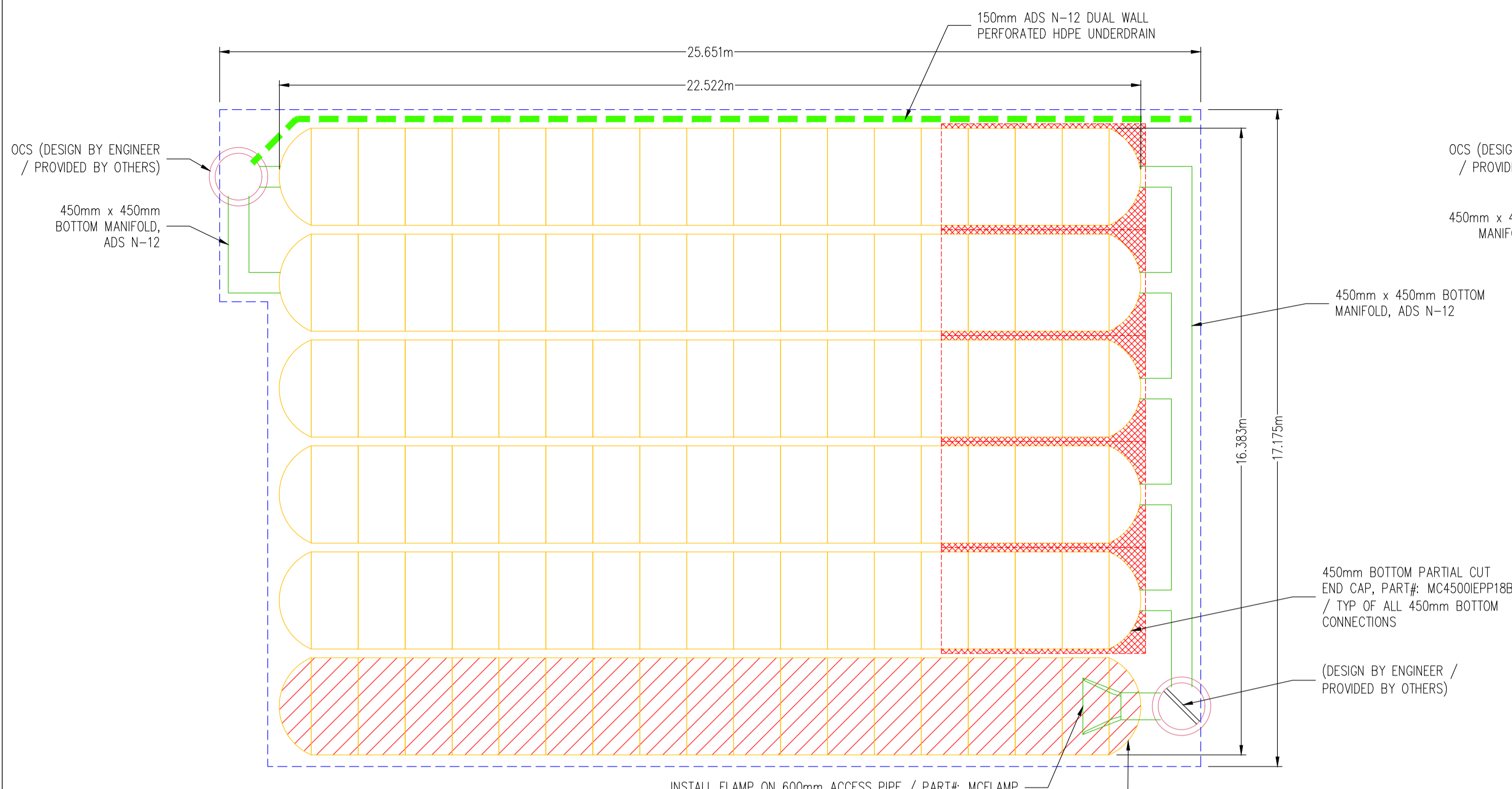
ATTENUATION TANK 1. REFER TO DRAWING D111-CSC-XX-XX-DR-C-0002_Proposed Drainage Layout SCALE 1:100
